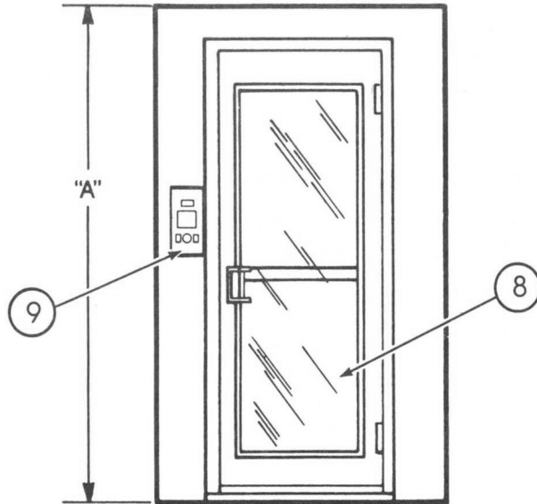
FRONT VIEW ENTRANCE
